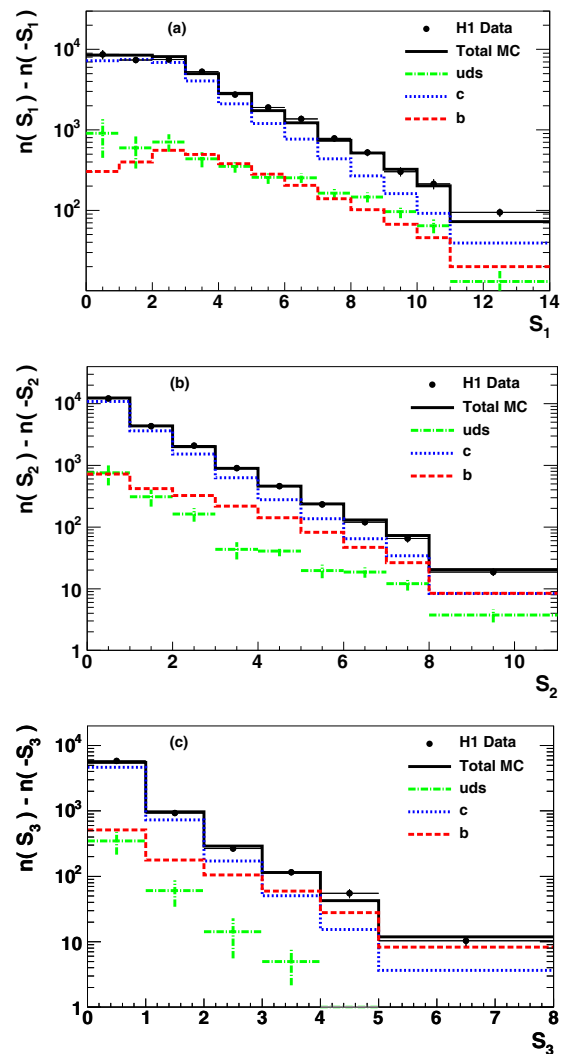
Fig. 4. The subtracted significance distributions of a S_1 , b S_2 c S_3 . Included in the figure is the result from the fit to the data of the Monte Carlo distributions of the various quark flavours
